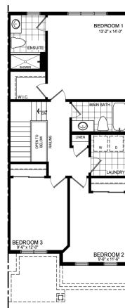
SECOND FLOOR PLAN STYLE A1
