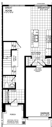
GROUND FLOOR PLAN STYLE A1
