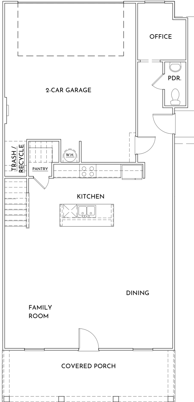
FIRST FLOOR
