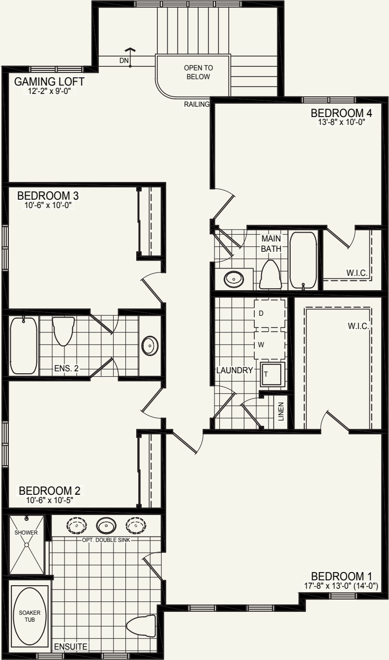
SECOND FLOOR PLAN STYLE A
