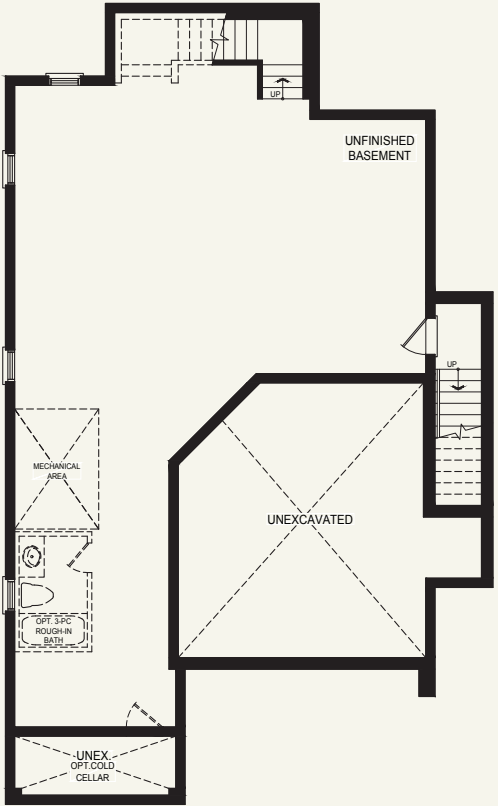
BASEMENT PLAN STYLE A
