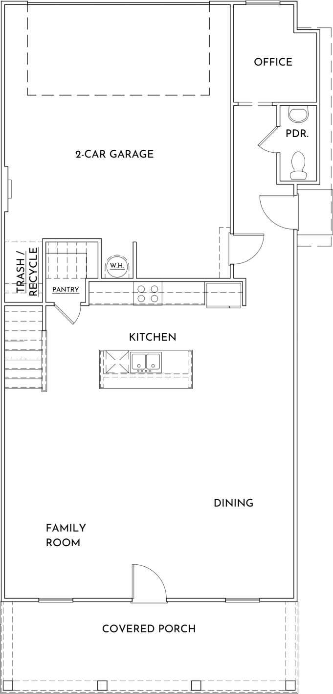
FIRST FLOOR
