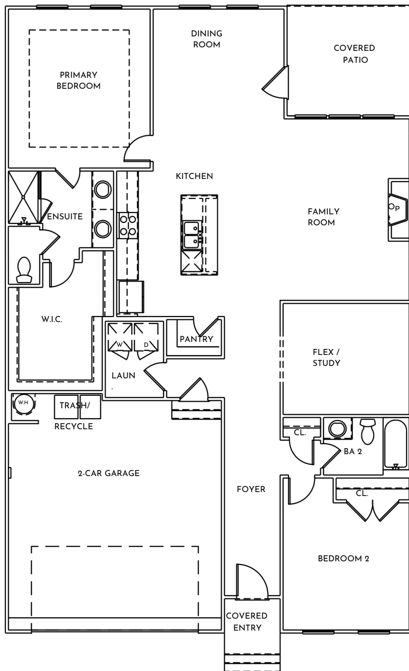
FIRST FLOOR
